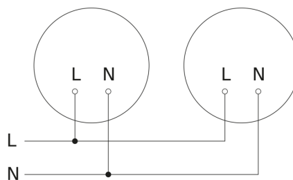
Master/master bluetooth interconnection circuit diagram
